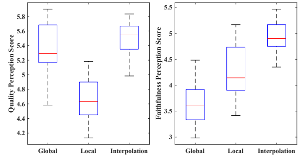
Fig. 16. Box plots of the average quality and faithfulness perception scores over the participants for each method.
