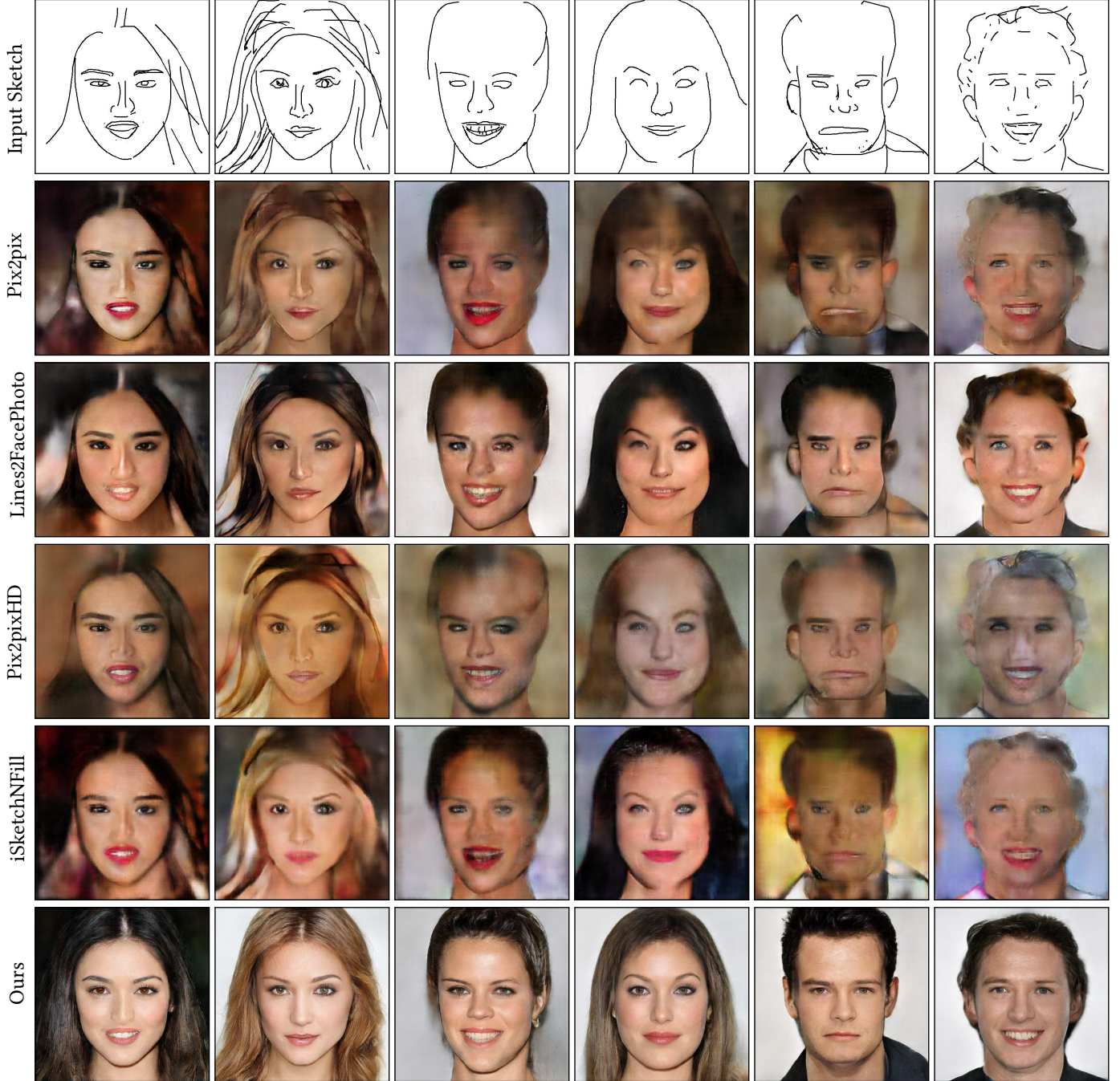
Fig. 17. Comparisons with the state-of-the-art methods given the same input sketches (Top Row).
