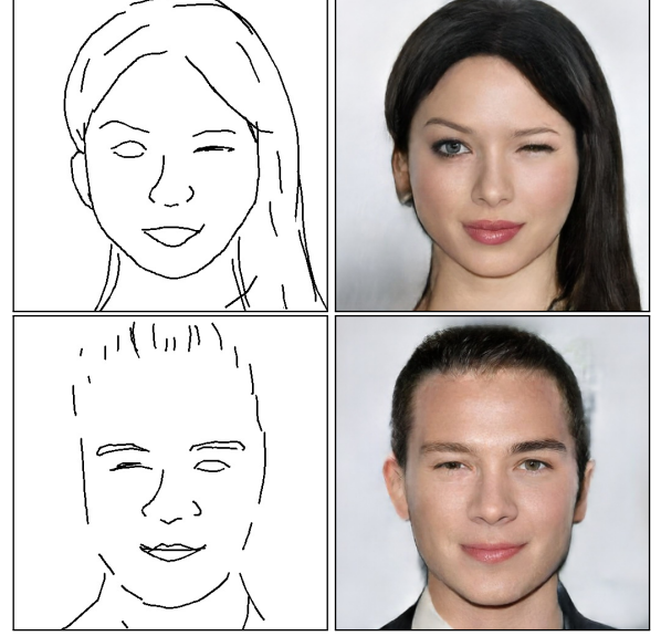
Fig. 4. Two examples of generation flexibility supported by using separate components for the left and right eyes.
