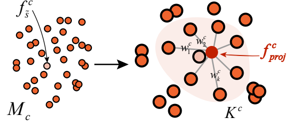
Fig. 6. Illustration of manifold projection. Given a new feature vector f_s^c , we replace it with the projected feature vector f_{proj}^c using K nearest neighbors of f_s^c .
